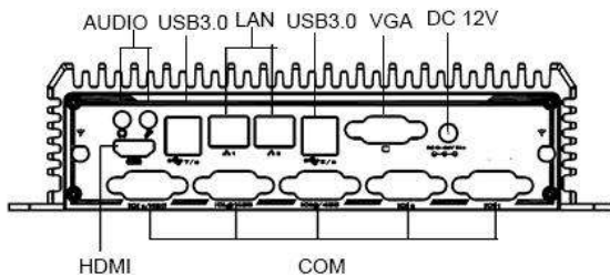
2: Rear IO interface
