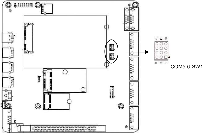
(C69-D6 Jumper postion)
