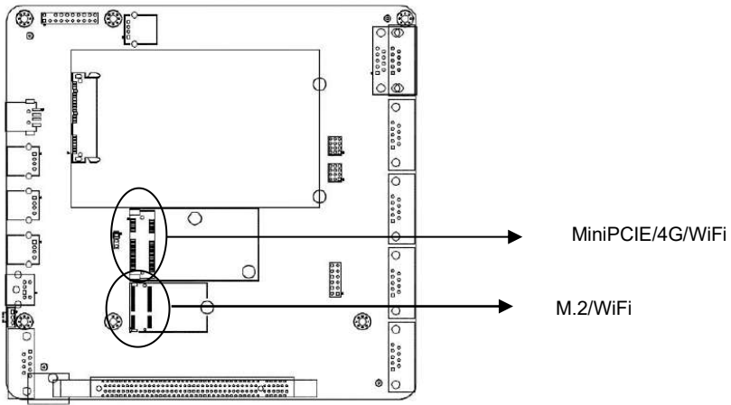
(C69-D6 M.2 and MINIPCIE slot position)
