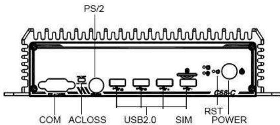
1: Front IO interface
