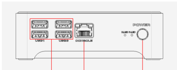
Front panel external I/O view
