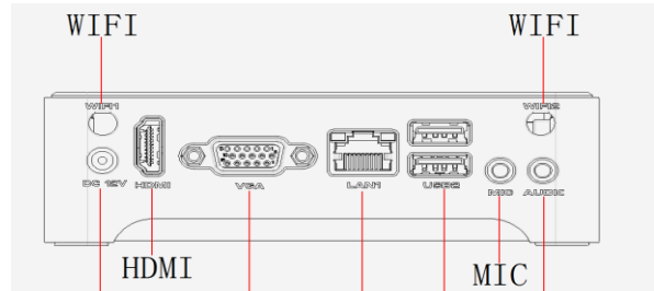
External I/O view of the rear panel
