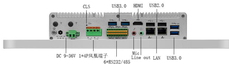
Bottom I/O View
