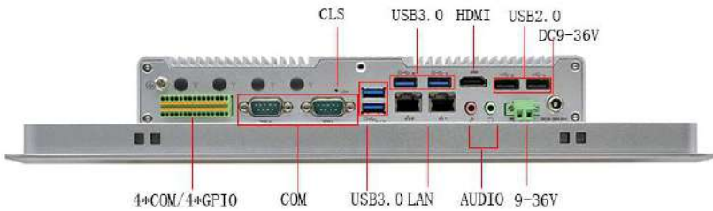
Image 2: Bottom IO View
