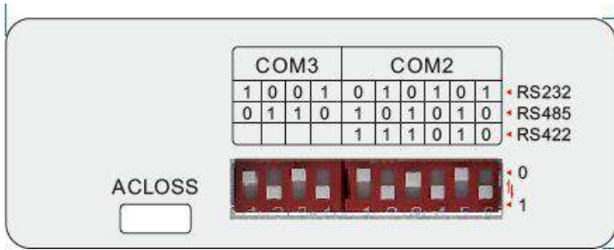
10-digit DIP switch image
