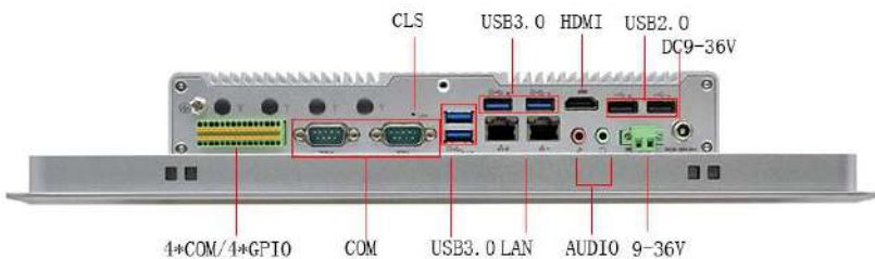
Image 3: Bottom I/O View
