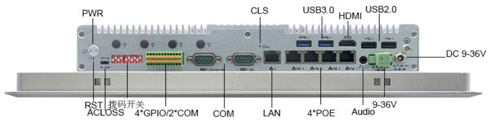
Bottom I/O View
