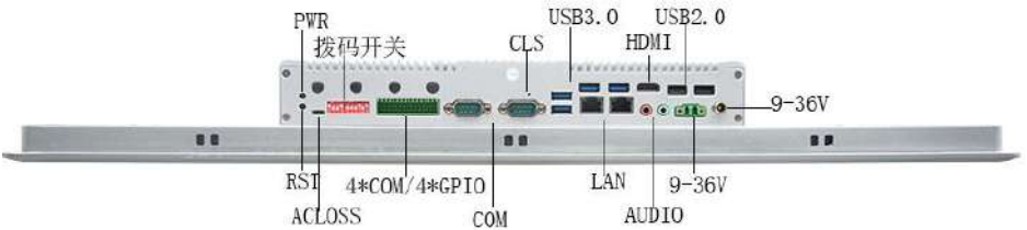
Image 3: P2381Y-C6 Bottom I/O View
